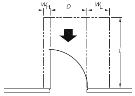
(f) Latch-side approach, door opens towards user
